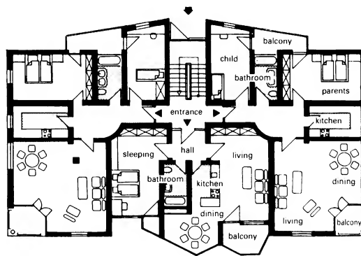
9 Three dwellings per floor
